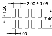
Recommended P.C.Board SMD Layout
